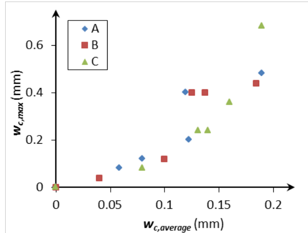
Figure 1. The relationship between the average and maximum crack widths.
